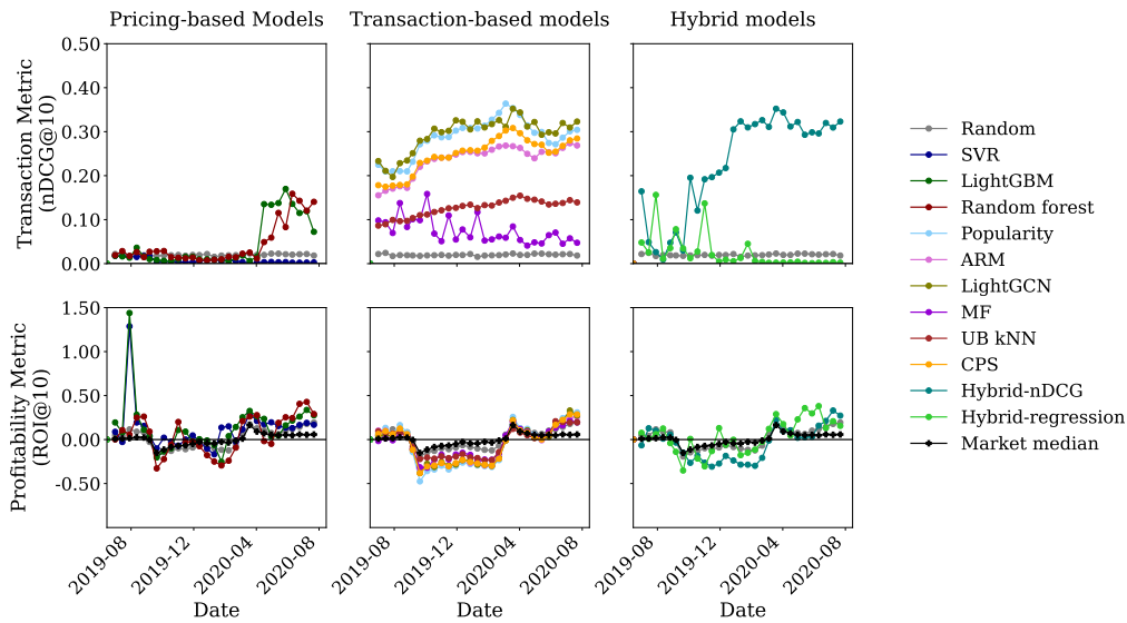
Figure 2: Comparison of performances reported by the Transaction-Based nDCG@10 and Profitability-based ROI@10 metrics for 12 recommendation algorithms over time.
